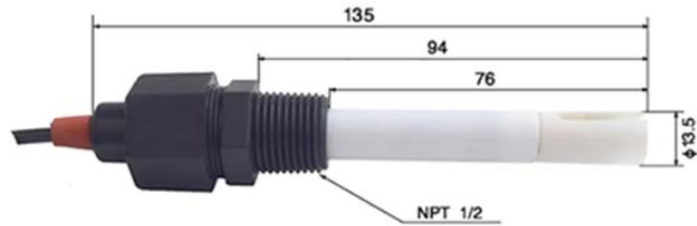
ABS conductivity electrode with 5m cable constant: K=1.0 Temperature: 0-50°C pressure: 0-0.5MPa
